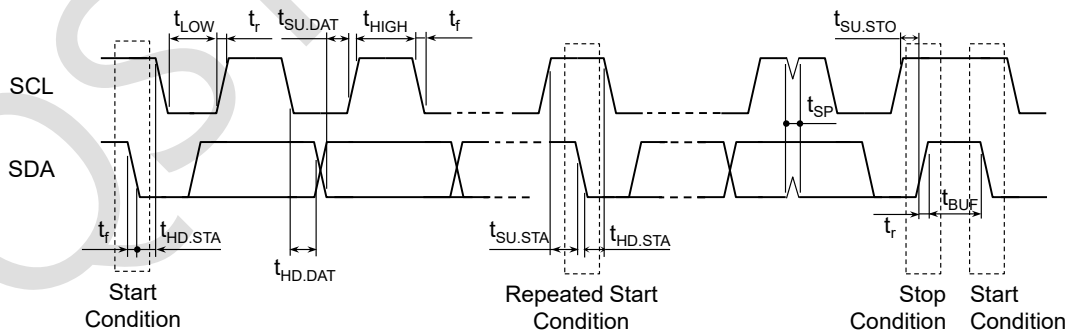
Timing Chart of the I 2 C
