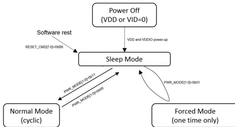
Figure 7: Mode transition diagram
