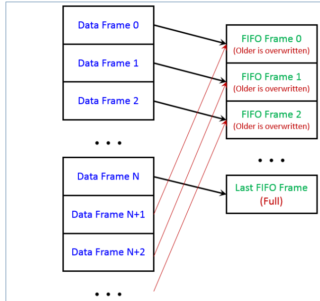
Stream Mode
