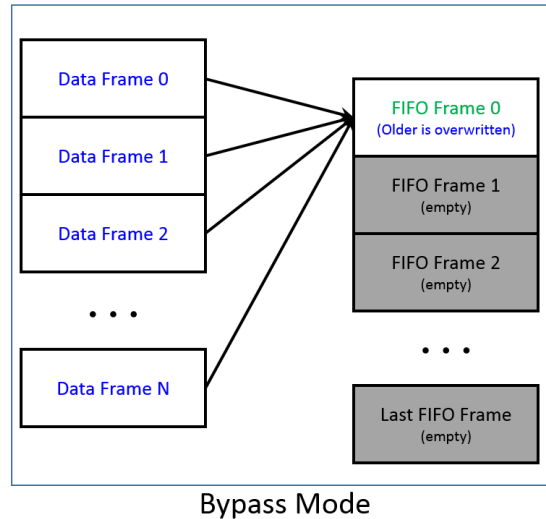
Figure 10: Bypass mode
