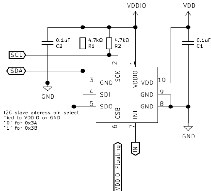
Figure 4: QMP6990 I 2 C Connection Example
