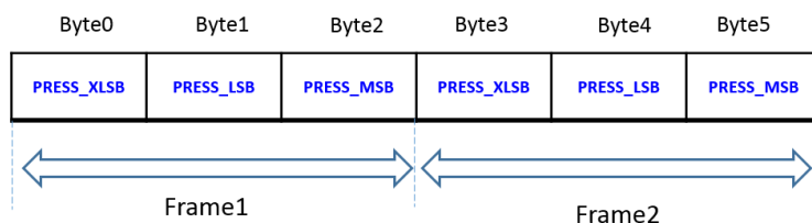
Figure 14: Frame format when only pressure is enabled
