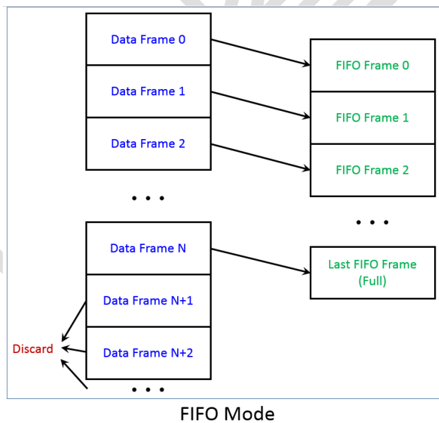
Figure 11: FIFO mode
