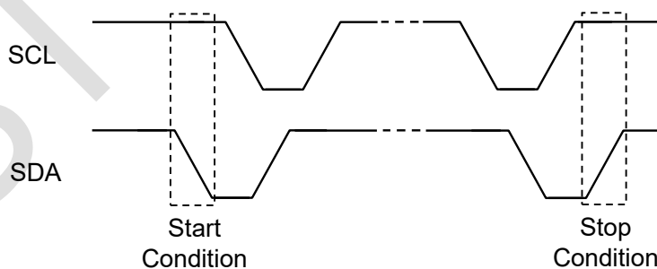
Figure 13: I 2 C START and STOP condition
